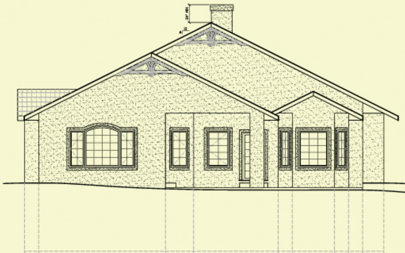
REAR ELEVATION
